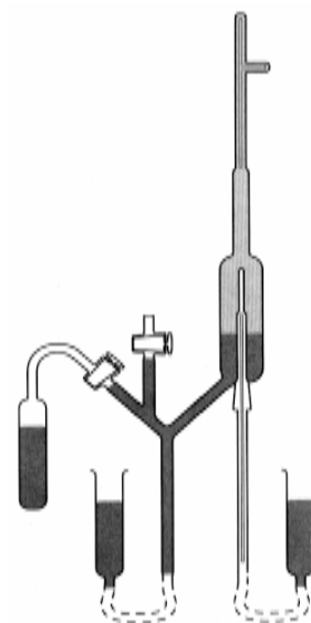
Proof alpha particle is helium
