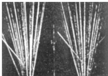
Cloud Chamber Track
